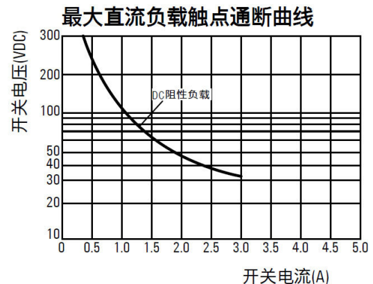
DC load limit curve Resistive load
