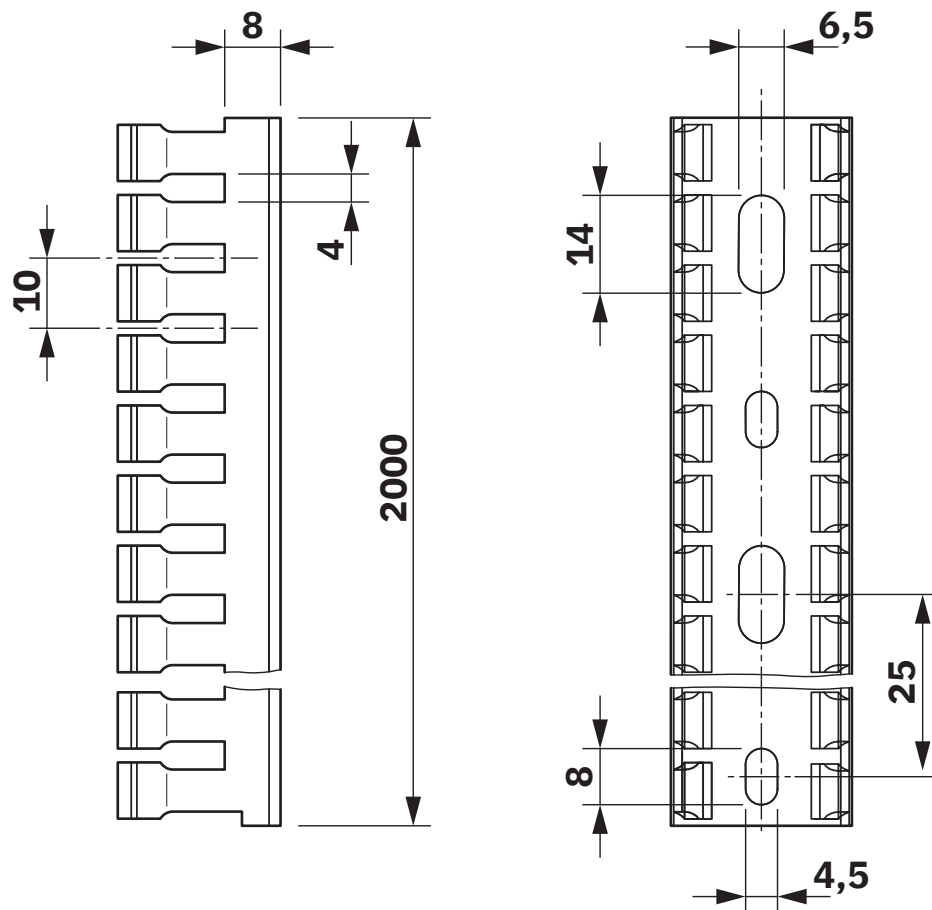
Dimensional drawing
