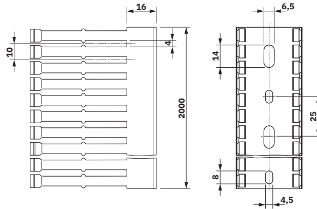
Dimensional drawing
