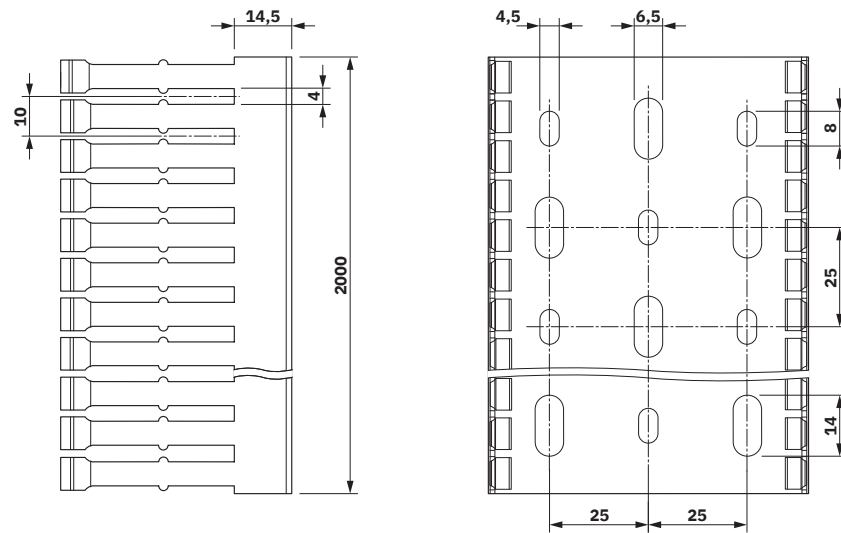
Dimensional drawing
