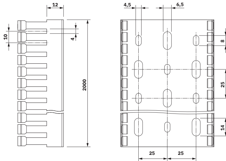
Dimensional drawing
