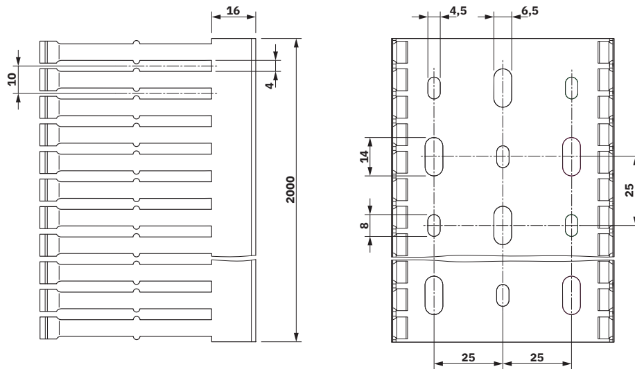
Dimensional drawing
