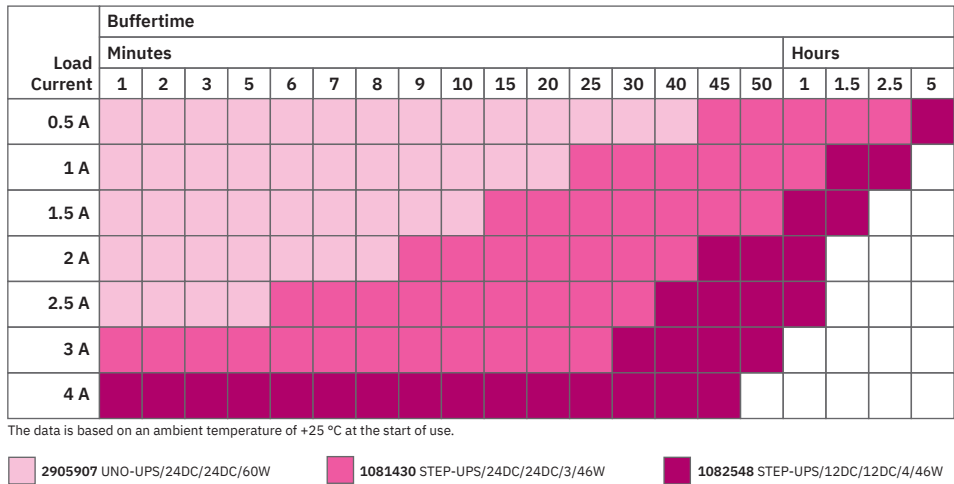
Buffer times for STEP DC UPS with integrated battery
