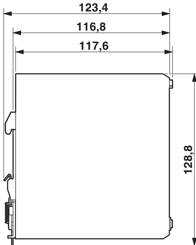
Dimensional drawing
